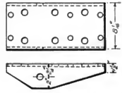
Figs. 251-252. Sling Stay Channel.
